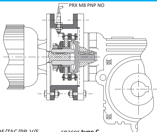
DF/TAC/PR-V/S → spacer type C (with sensor) (with inspection)
